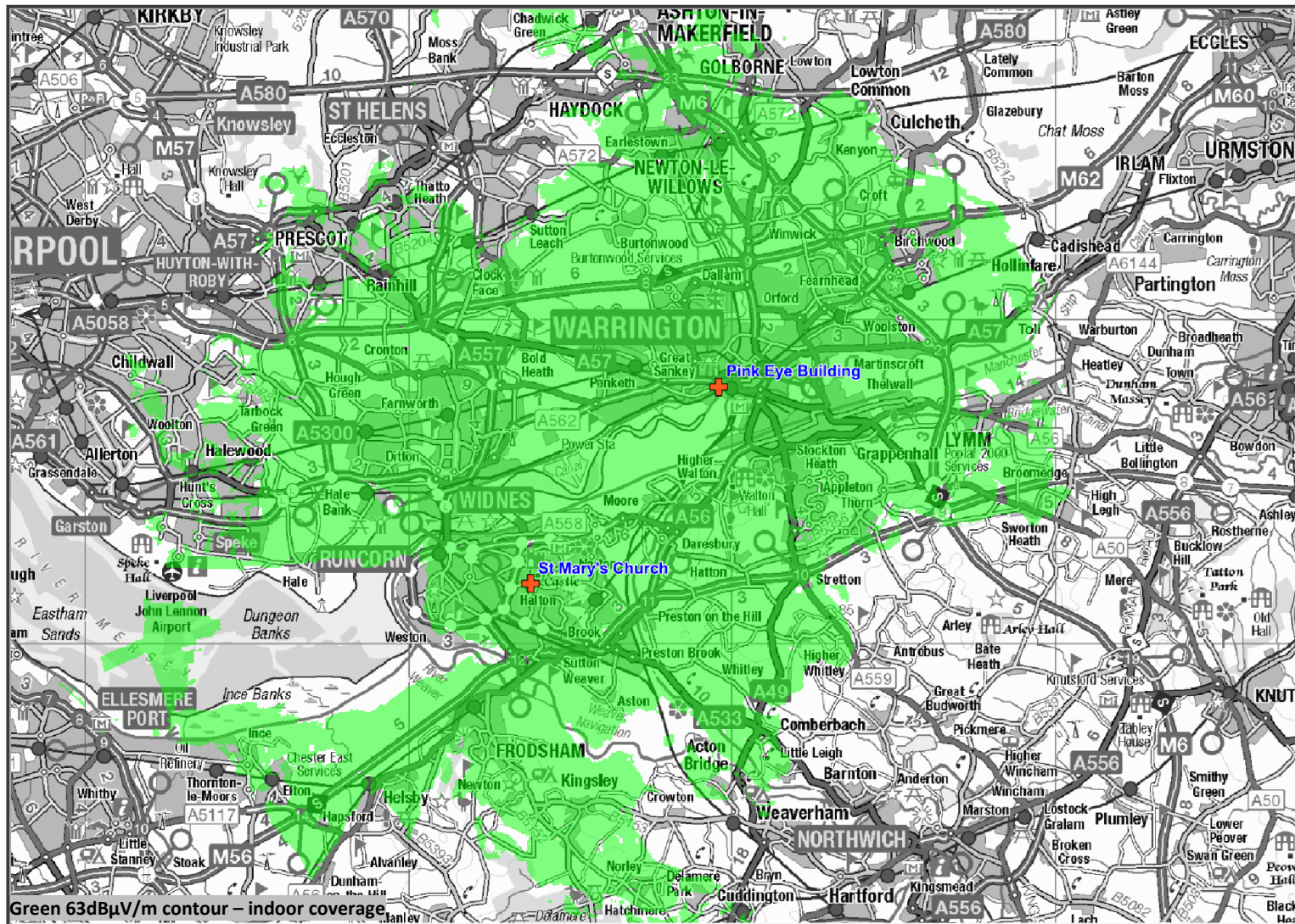
Figure 1: Predicted indoor coverage of the Warrington Widnes and Runcorn small-scale DAB multiplex. November 2023
