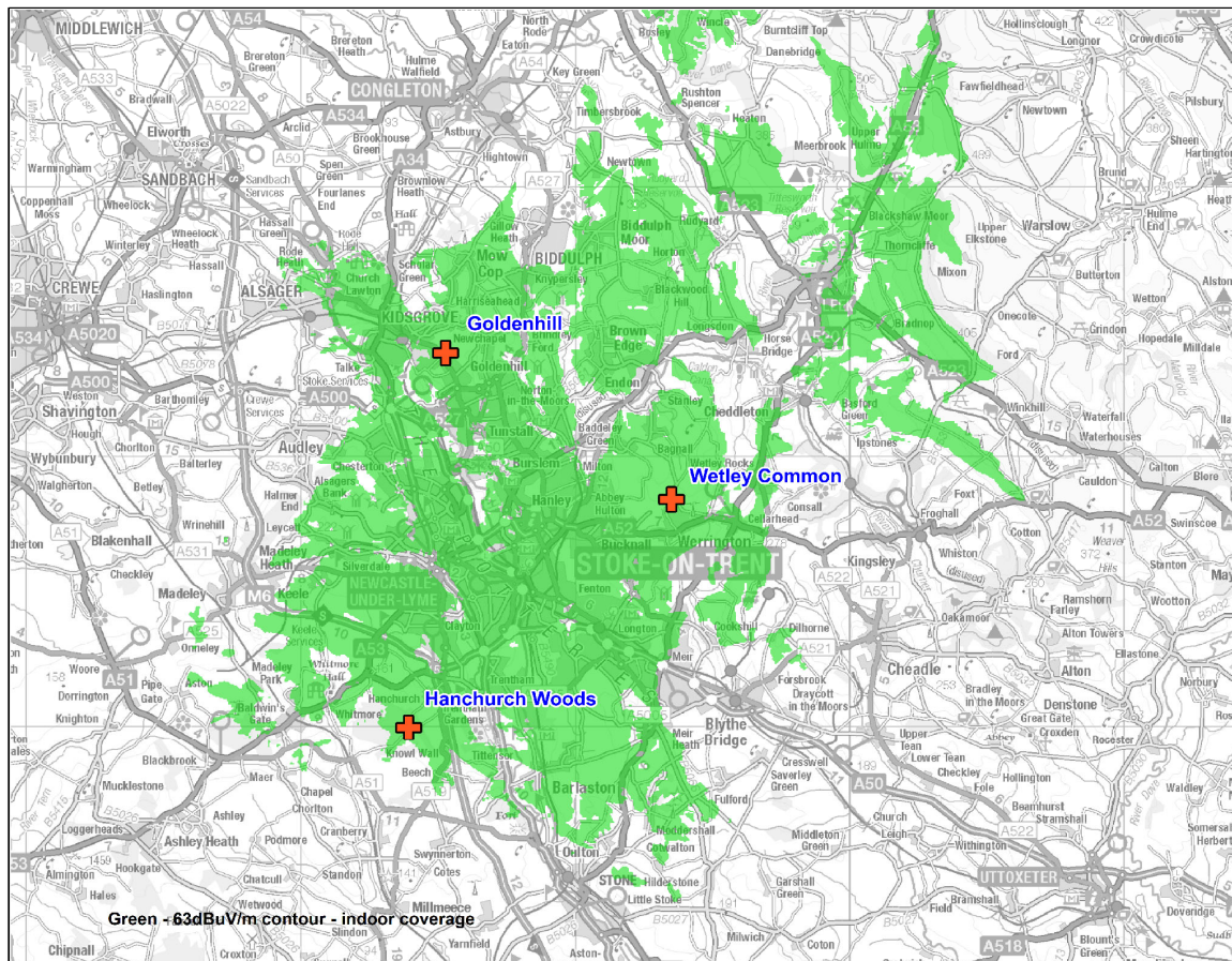
Figure 1: Predicted indoor coverage of the Stoke & Newcastle small-scale DAB multiplex. November 2023
