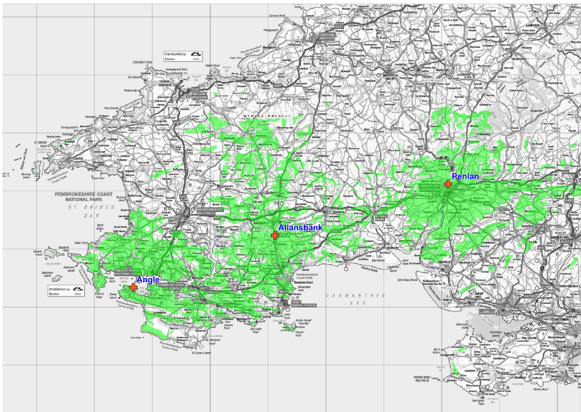
Figure 1: Predicted indoor coverage of the South Pembrokeshire small-scale DAB multiplex. July 2024
