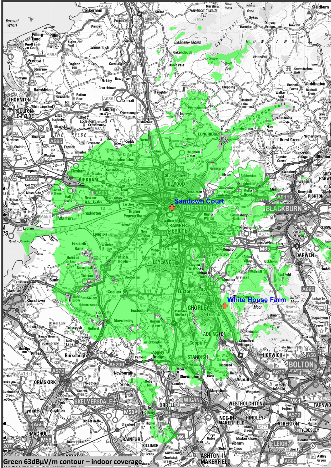
Figure 1: Predicted indoor coverage of the Preston small-scale DAB multiplex. November 2023
