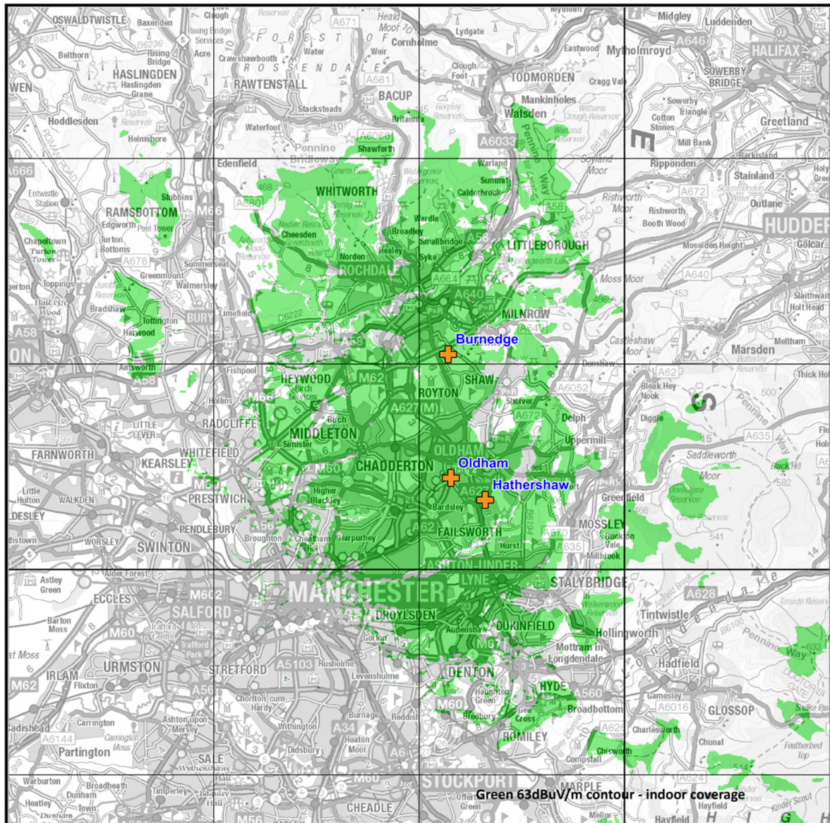
Figure 1: Predicted indoor coverage of the Oldham & Rochdale small-scale DAB multiplex. November 2023
