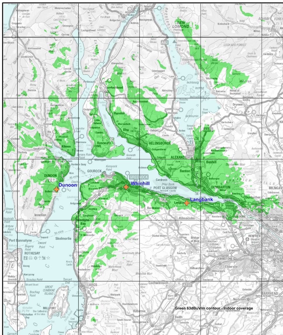
Figure 1: Predicted indoor coverage of the Inverclyde small-scale DAB multiplex. August 2024.
