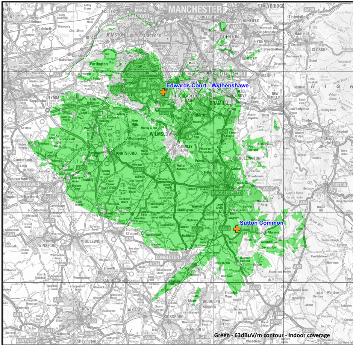
Figure 1: Predicted indoor coverage of the Cheshire East small-scale DAB multiplex. November 2023
