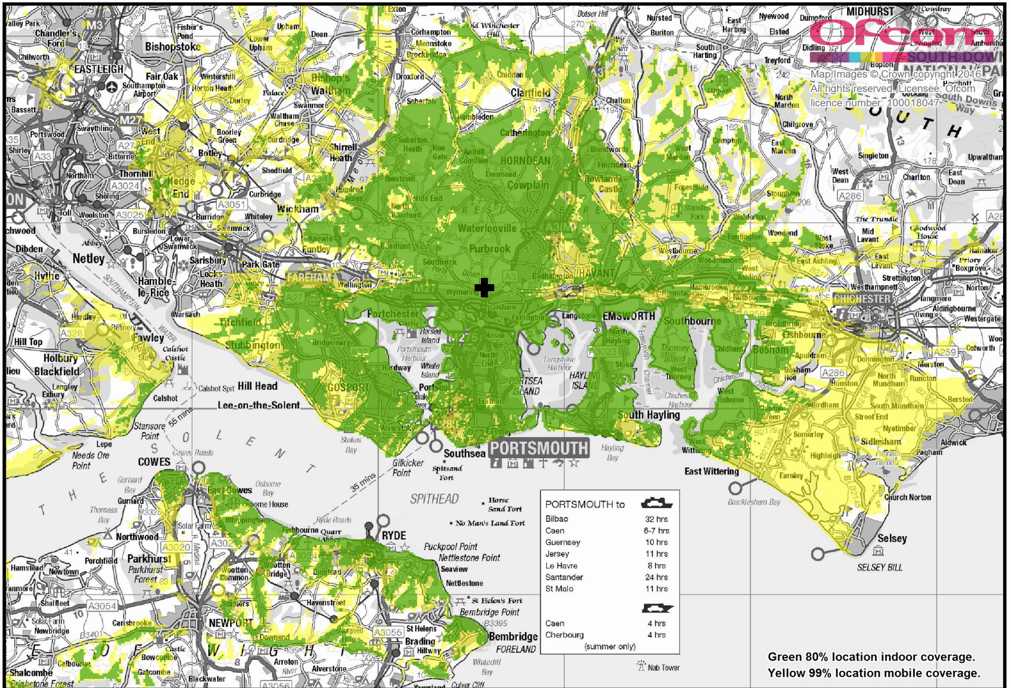
Portsmouth small scale DAB trial predicted coverage. April 2016.
