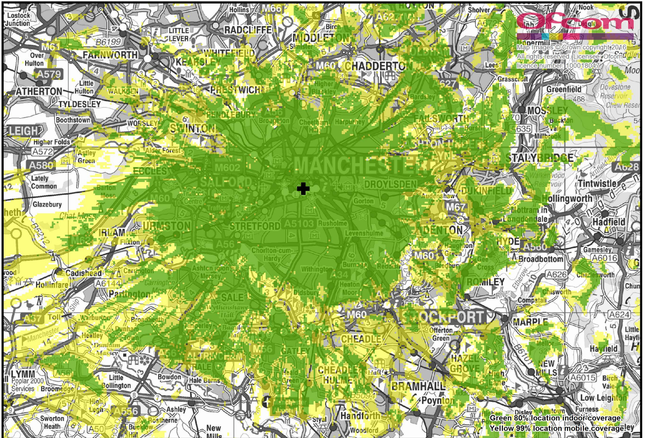
Manchester small scale DAB trial predicted coverage. April 2016.
