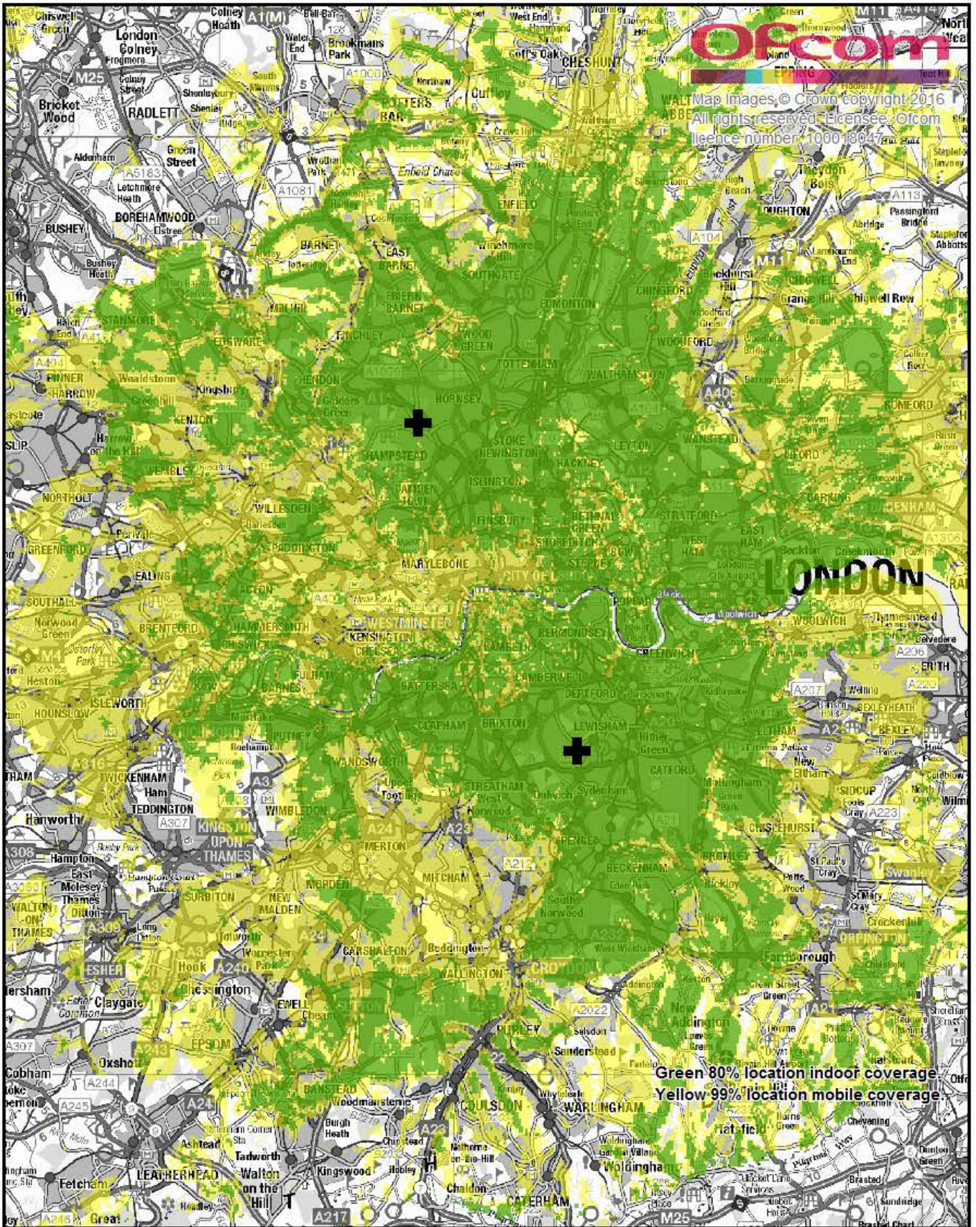
Central London small scale DAB trial predicted coverage. April 2016.
