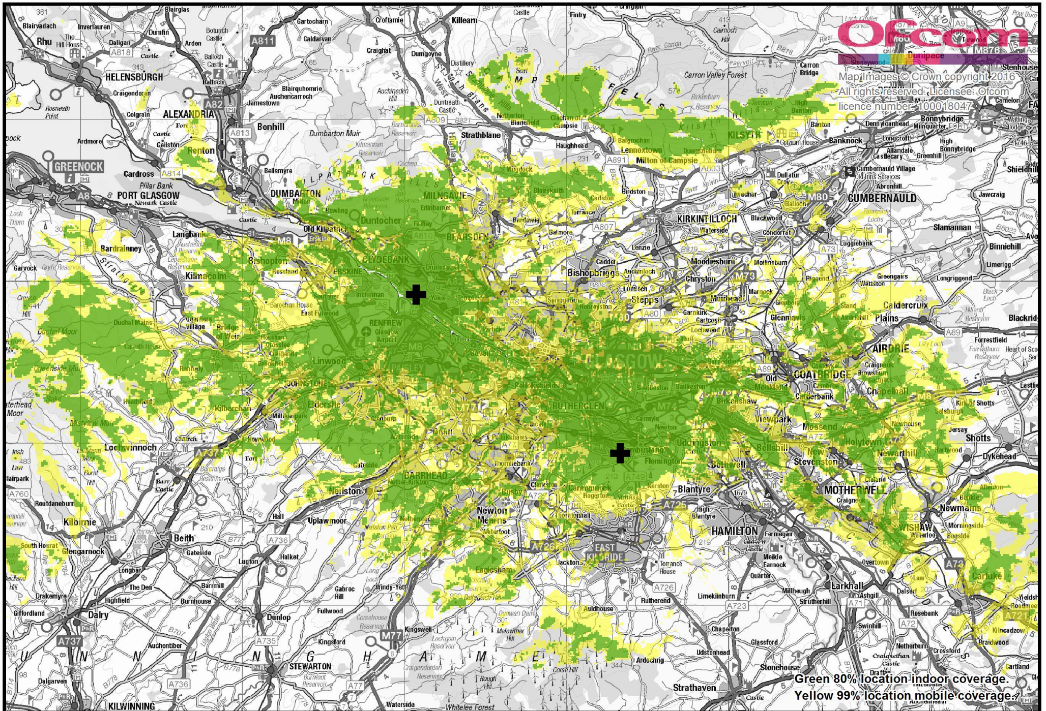
Glasgow small scale DAB trial predicted coverage. April 2016.
