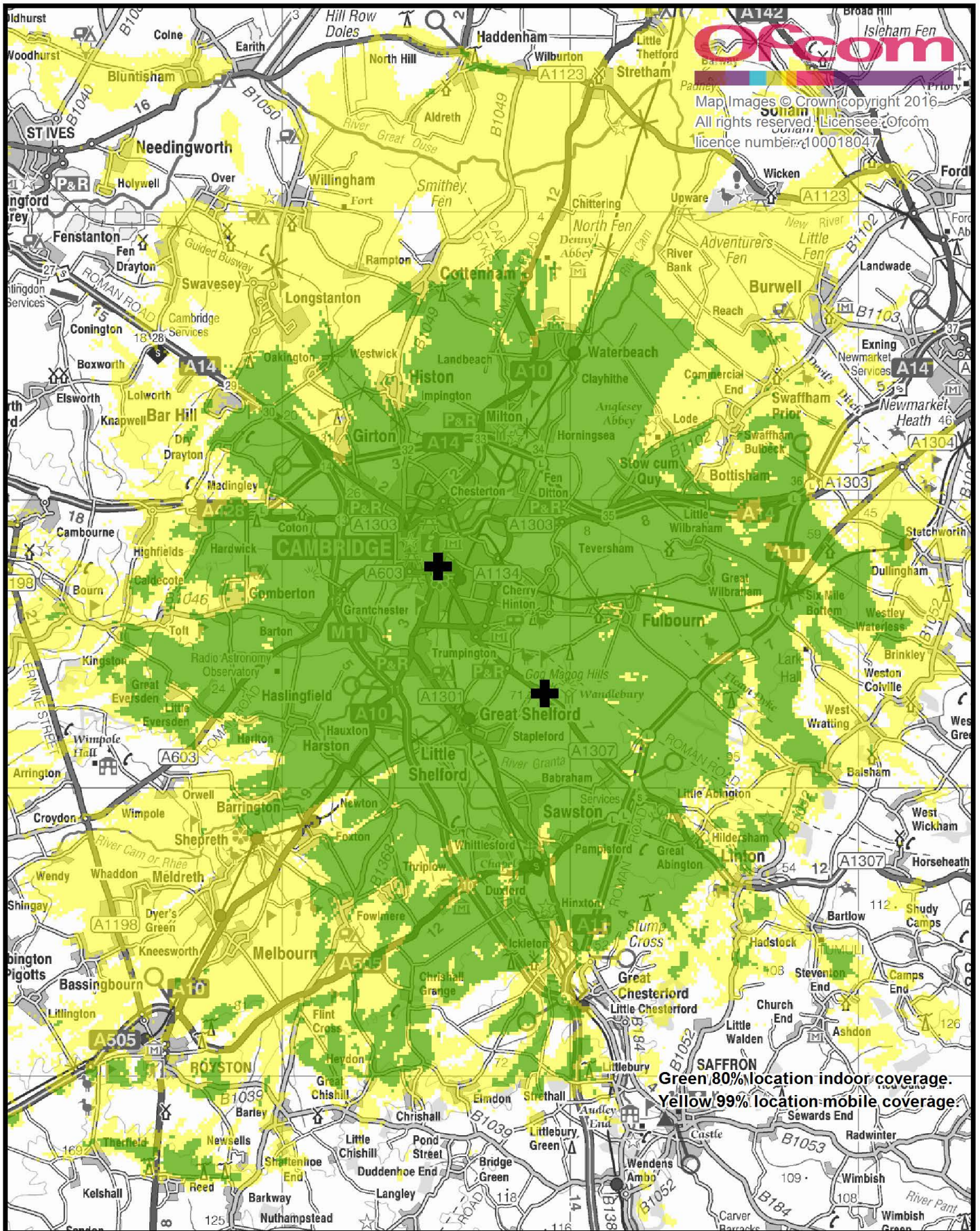
Cambridge small scale DAB trial predicted coverage. April 2016.
