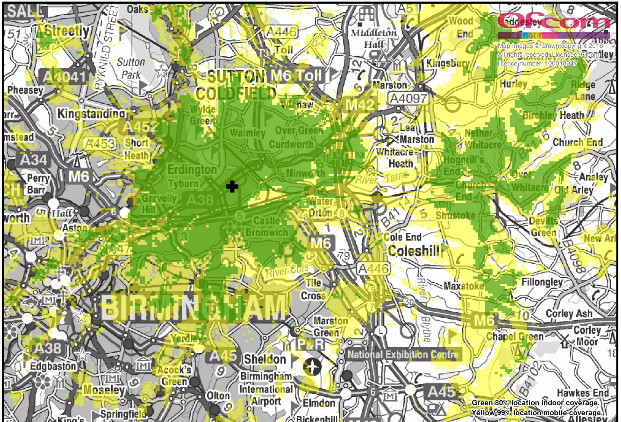
North East Birmingham small scale DAB trial predicted coverage. April 2016.
