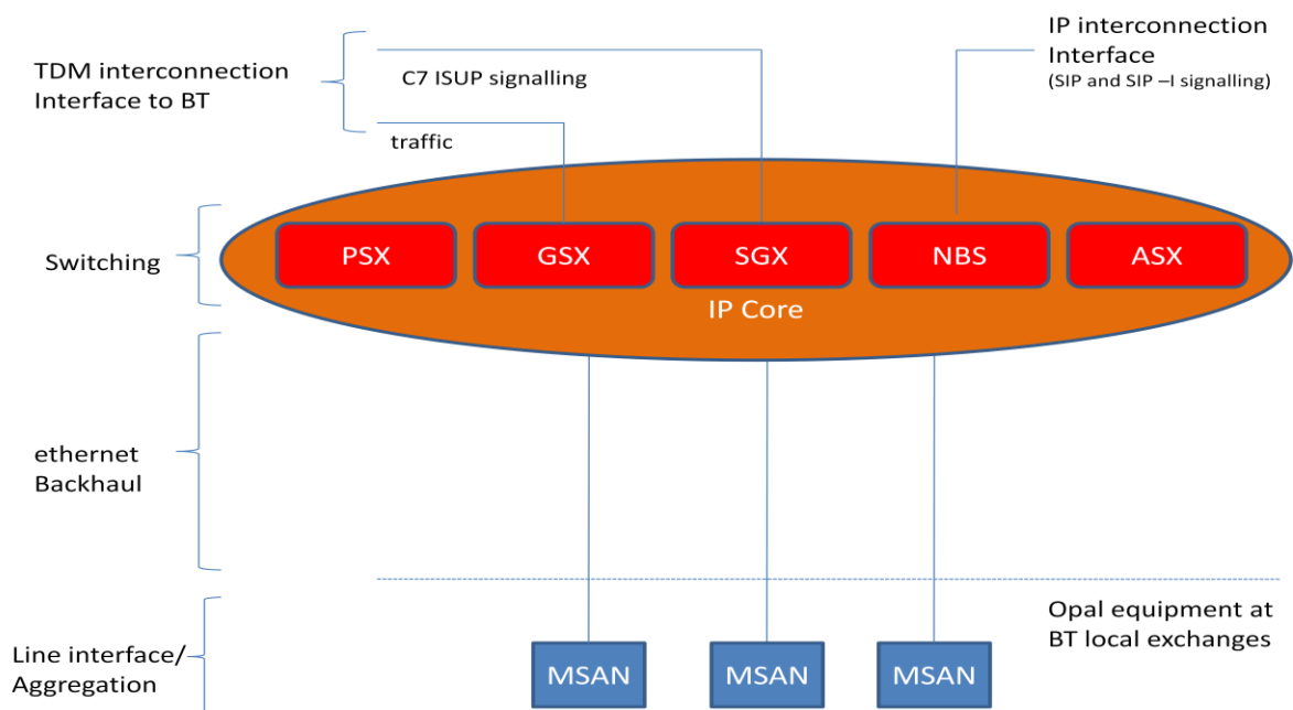
Figure 5: Ofcom view of Opal NGN Network Architecture
