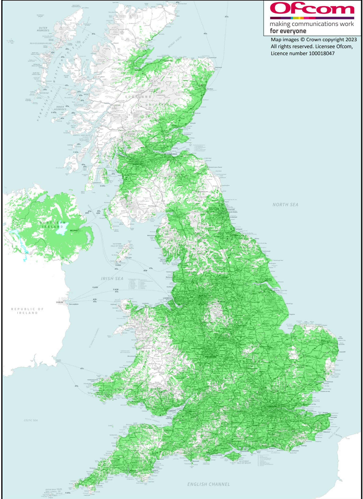
D1 noise limited coverage 80% location (63dBuV/m coverage contour) - Adult population served 48,621,898
